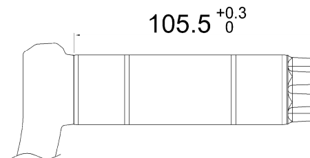
Fig.1 Spindle dimension (w/o Preload Nut ④)
