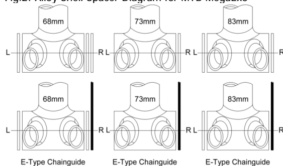
Fig.2: Alloy Shell Spacer Diagram for MTB MegaExo
