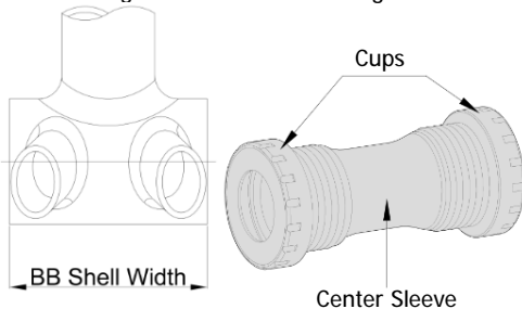
Fig.2: Alloy Shell Spacer Diagram for MTB MegaExo
