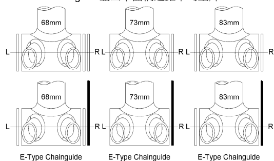
Fig.2: 登山車曲柄之鋁華司墊片
