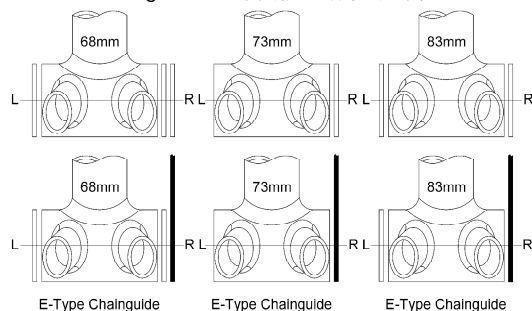
Fig.2: 登山车曲柄之铝华司垫片
